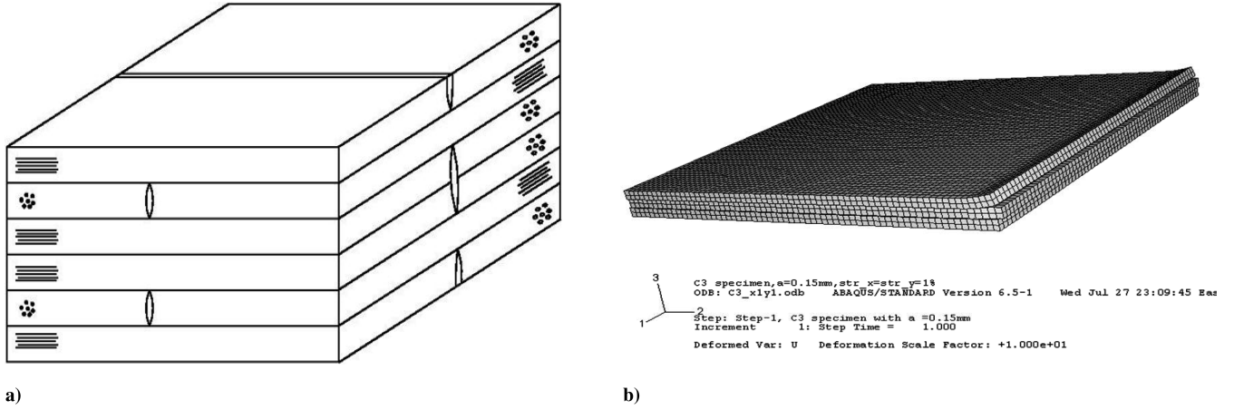
Fig. 13 Geometric model and typical deformation for multiple-layer laminates.
